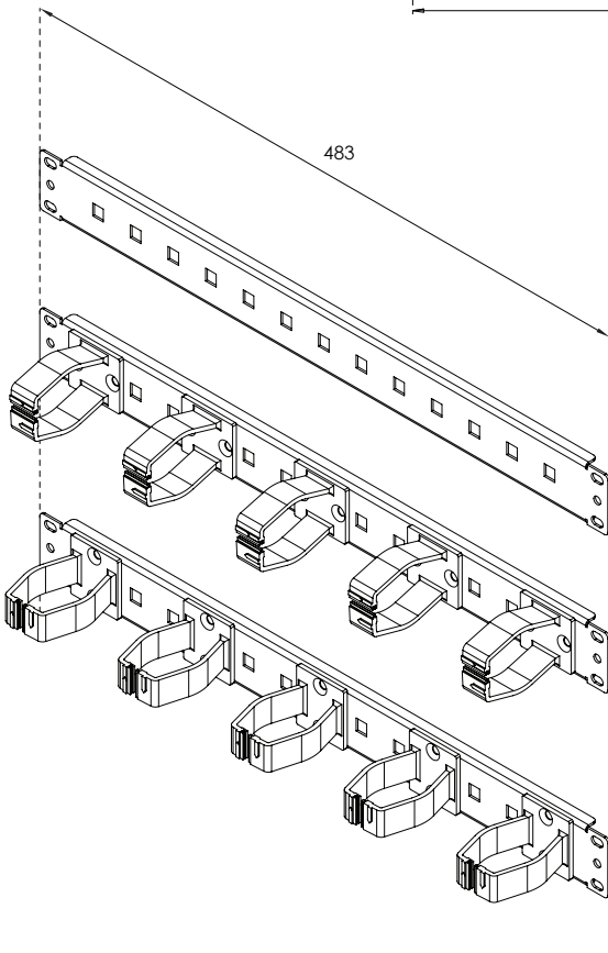
Front Panel
