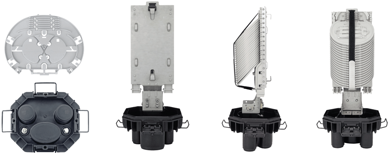
Single Circuit Tray | Thickness: 4mm 6 Splices Capacity
